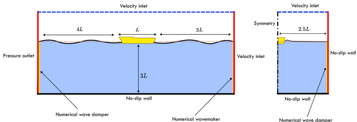
Fig. 46. CFD domain used for solving the fluid flow around a flexible ship. The dimensions are set to be equal to those set by Lakshmyraranana and Hirdaris (2020). Here, L denotes the length between perpendiculars.
