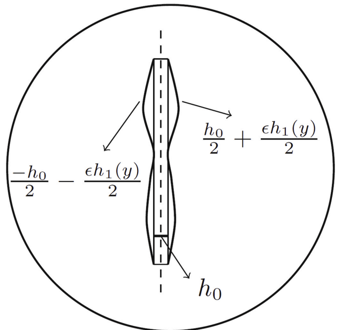
Fig. 30. Perturbed flexible thin plate with thickness d(y) = h_0 + h_1(y) ; Singh and Gayen (2023a) . © Elsevier.
