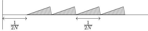
FIGURE 3. An illustration of the translated copies \Delta_k^i of \Delta_k .
