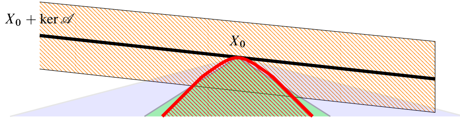
FIGURE 3.1. Geometric illustration of our approach: Close to X_0 the descent set (indicated by the red line) is near-tangential to the kernel of the measurement operator \mathcal{A} , so the descent cone (light blue) is rather wide. By restricting to noise levels above a certain threshold we only need to cover the descent set at some distance, which is achieved by a much smaller cone (green). Note that below the noise level (orange strip), the green cone does not contain the full descent set.
