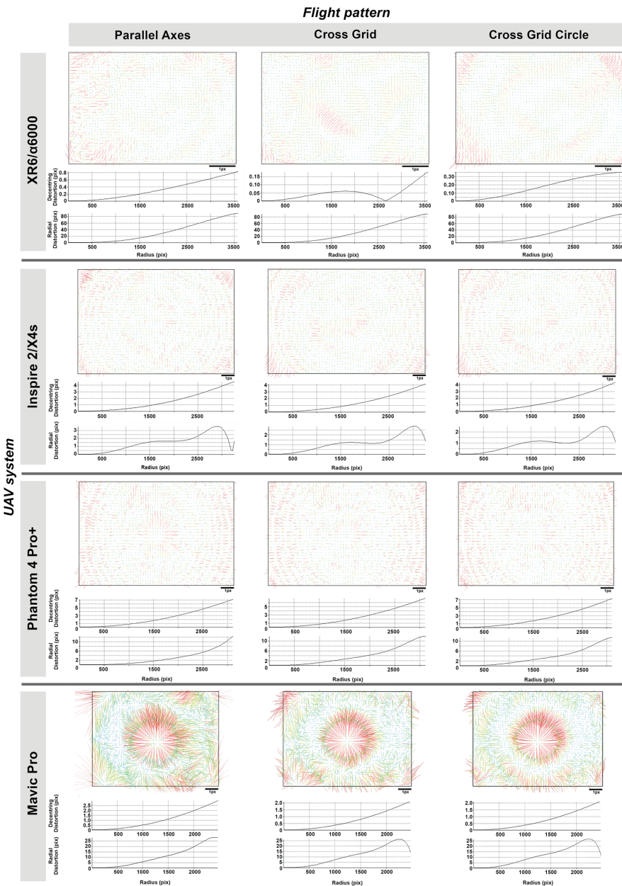
FIGURE A1 Camera residuals after autocalibration with decentering and radial distortion plots. Note the non-uniform scaling of the Y-axes in distortion plots [Color figure can be viewed at wileyonlinelibrary.com]
