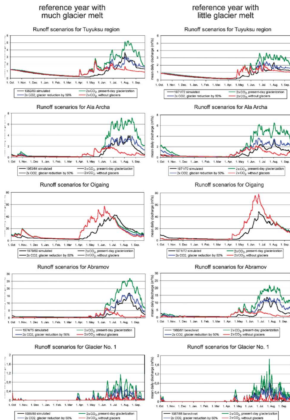
Figure 4 Calculated daily discharge of the reference year and of a climate scenario after the doubling of \text{CO}_2 (predicted by the GISS model), for three different steps of deglaciation
