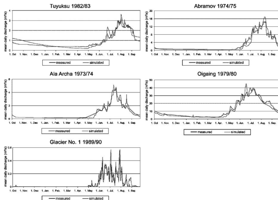
Figure 3 Comparison between measured and simulated daily discharge for one example year in each test area
