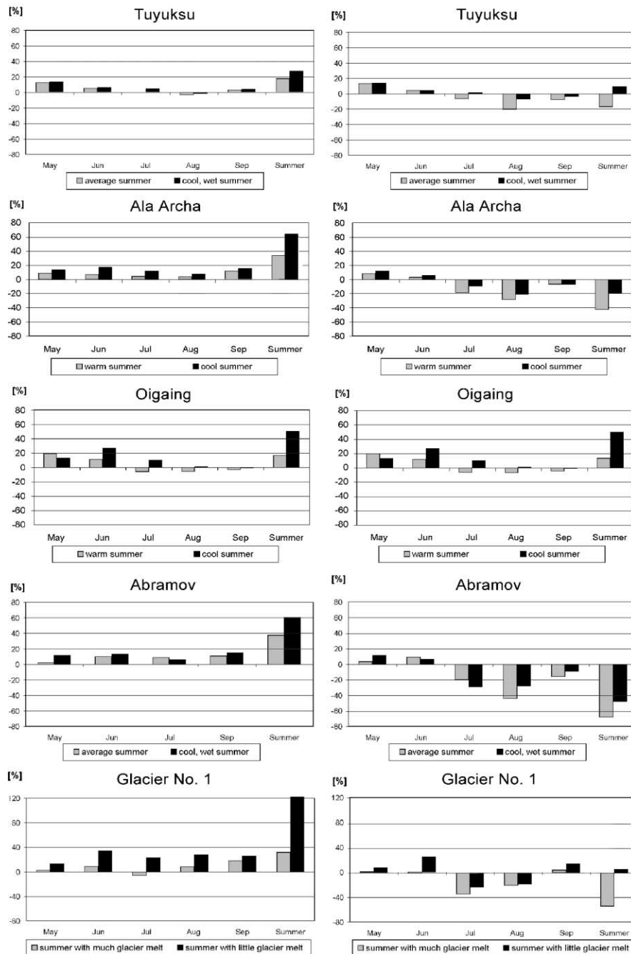
Figure 5 Effect of climate change (predicted by the GISS model for the doubling of \text{CO}_2 ) and glacier degradation on monthly discharge, related to summer runoff of the two reference years
